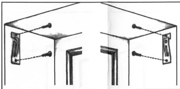
SPRING ROLLER - STANDARD ROLL BRACKET #163L
