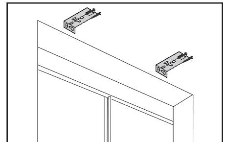
Outside Mount
