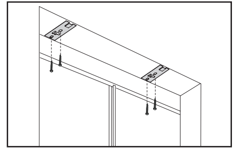
Inside Mount
